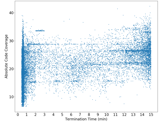
Fig. 3: Absolute Code Coverage vs Termination Time
